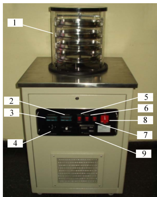
Figure 1: Rificor Freeze Dryer model L-A-B4-C. 1. Vacuum chamber; 2. Shelf temperature control; 3. Display showing either shelf, product or condenser temperature; 4. Switch to select the temperature being displayed; 5. Switch that starts the condenser and its temperature measurement; 6. Switch for starting the vacuum pump and pressure gauge; 7. Switch to start heating the shelves; 8. Main switch; 9. Absolute pressure gauge.
